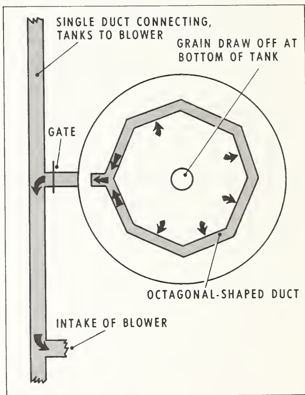
FIGURE 1.—Top view of the duct system.
